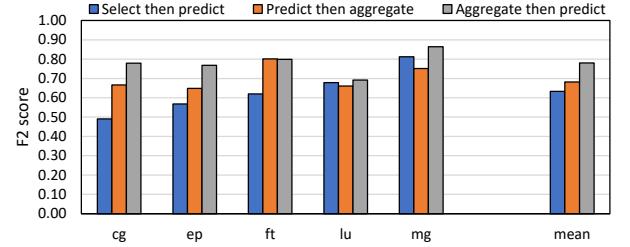
(a) Comparing different approaches for handling multi-node applications
