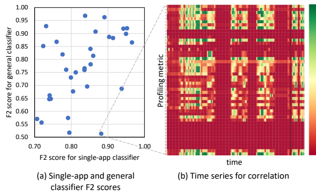
Figure 6: Single-application vs. general classifiers
