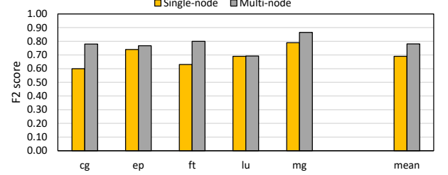
(b) Comparing prediction quality for single- and multi-node versions of the same application
